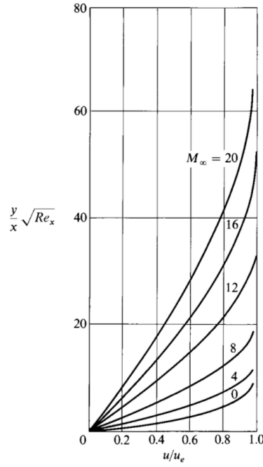
Figure 2.15: (Sutherland's Law effect on Laminar Boundary Layer Insulated Flat Plate).
