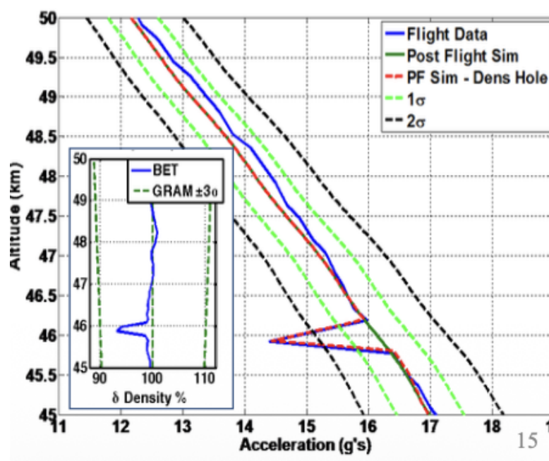
Figure 4.1: IRVE-3 Post-Flight Simulation vs. Flight Data for Acceleration and Density.
